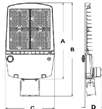
Trunnion mount A. 19 1/4" B. 22 1/8" C. 10 7/16" D. 3 1/4"
